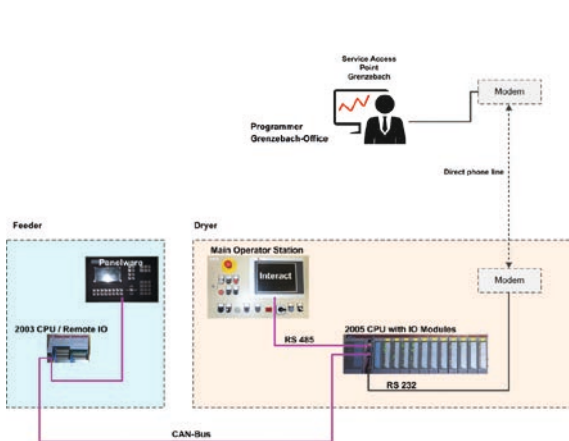
Old system architecture
