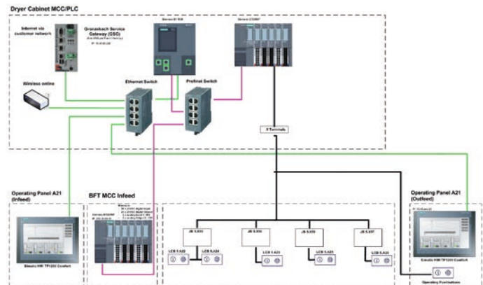
New system architecture with Siemens control components (with or without field I/Os)
