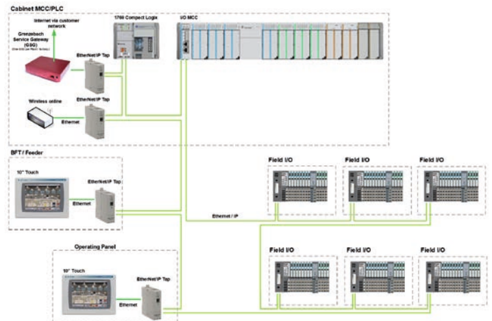
New system architecture with Rockwell control components (with or without field I/Os)
