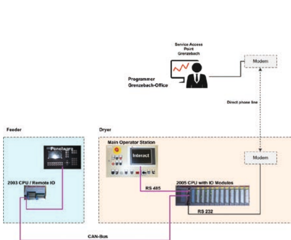
Old system architecture
