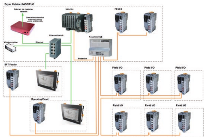
New system architecture with B&R X20 control components (with or without field I/Os)
